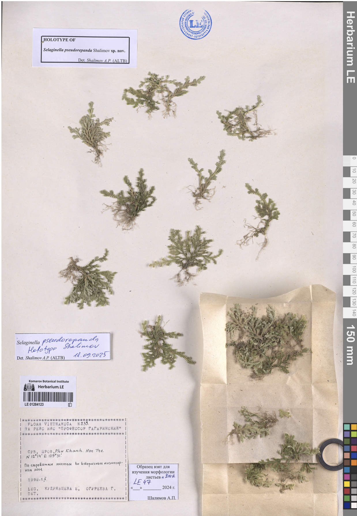
Fig. 3. Selaginella pseudorepanda Shalimov, sp. nov. Digitized images of holotype: E. Kudryavtzeva, G. Ogureeva No. 233 (LE 01284123).
