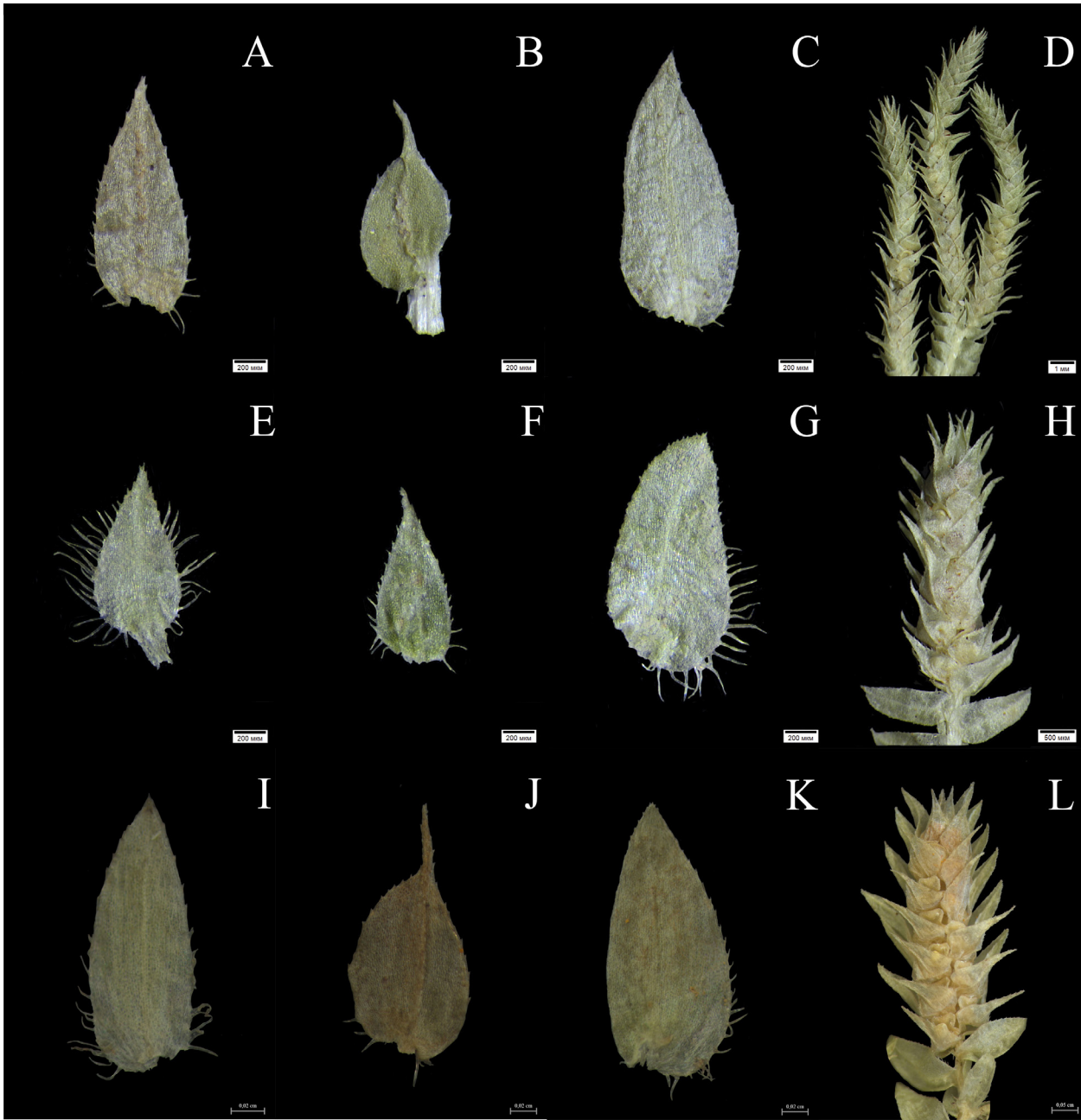
Fig. 5. Leaves and strobili of Selaginella repanda , S. pseudorepanda , and S. kurzii : A–D – Selaginella repanda (L. Averyanov et al. VH 1566, LE); E–H – S. pseudorepanda (E–G from the holotype of E. Kudryavtzeva, G. Ogureeva 233, LE 01284123; H – from the paratype S. Tagane et al. No. 304, VNM00072393); I–L – S. kurzii (F. G. Dickason 8164, LE: A, E, I – axillary leaves; B, F, J – dorsal leaves; C, G, K – ventral leaves; D, H, L – strobili. Scale bars = 200 µm (A, B, C, E, F, G, I, J, K), 1 mm (D), 500 µm (H, L).
