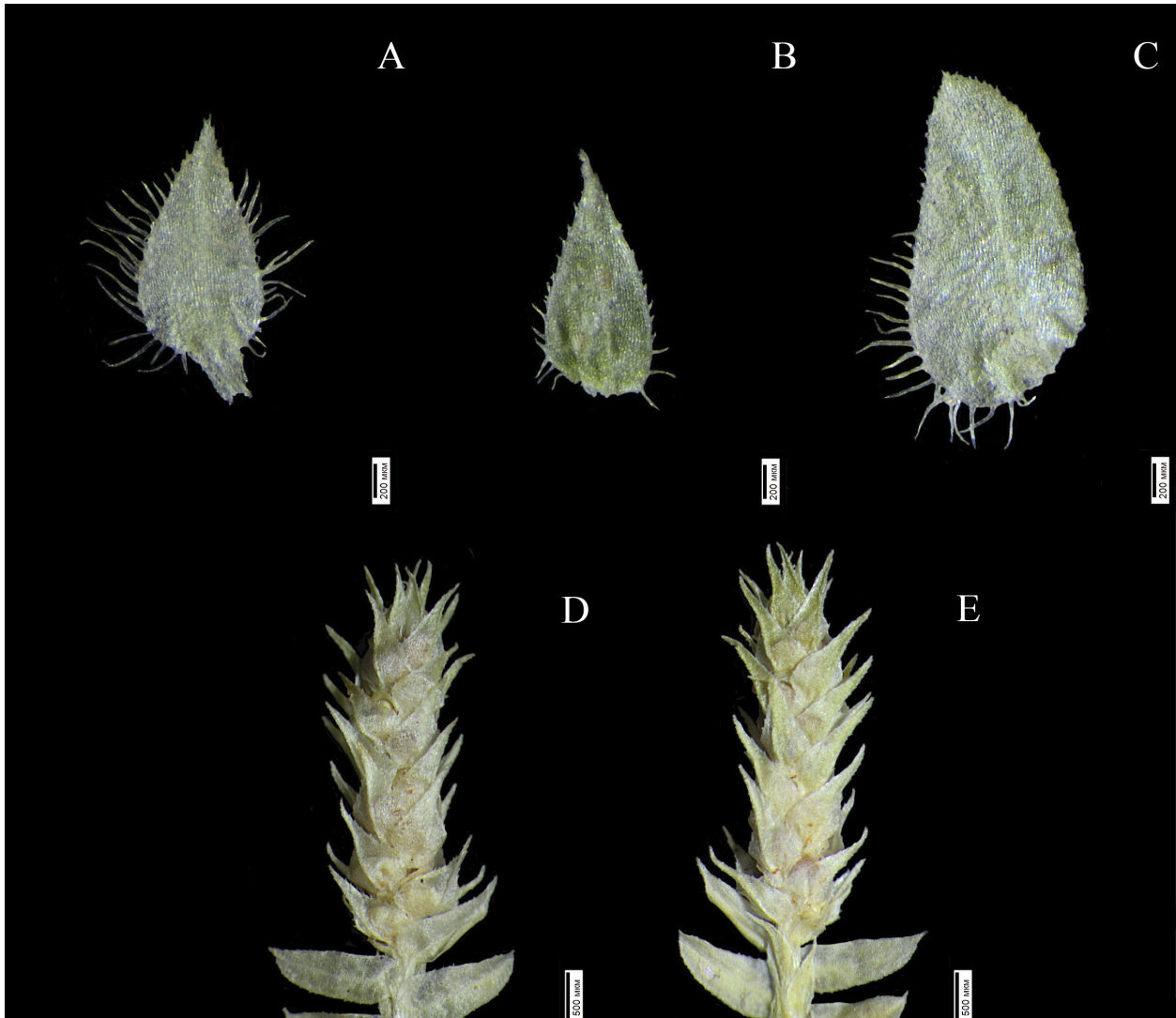
Fig. 4. Selaginella pseudorepanda Shalimov: A – axillary leaf, lower surface; B – dorsal leaves, upper surface; C – ventral leaf, lower surface; D – strobilus, lower surface; E – strobilus, upper surface; A–C – scalebar = 200 \mu\text{m} ; D, E – scalebar = 500 \mu\text{m} . A–C – taken from the holotype E. Kudryavtzeva, G. Ogureeva 233 (LE); D, E – taken from the paratype S. Tagane et al. No. 304 (VNM00072393).
