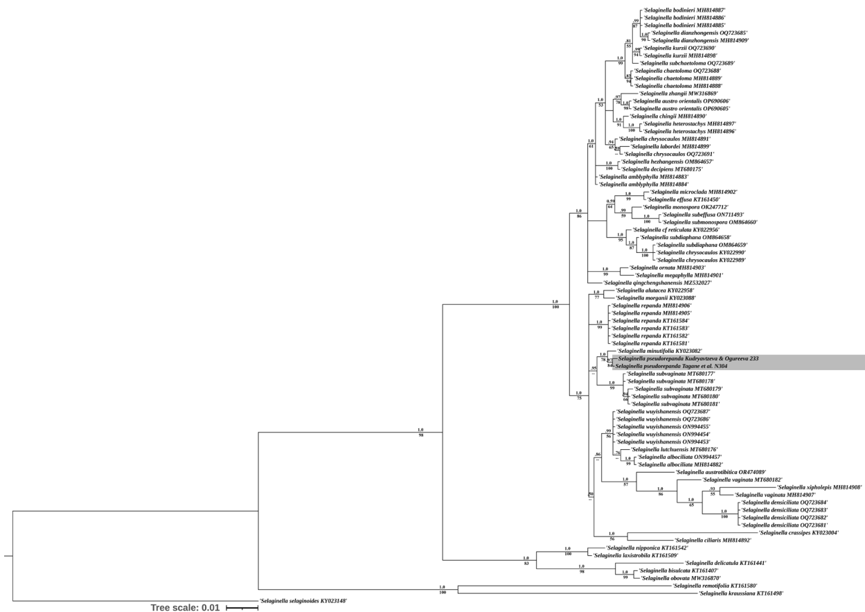
Fig. 1. The Bayesian inference (BI) tree of the new species and related species. Bayesian posterior probabilities and bootstrap supporting values calculated by maximum likelihood (ML) analysis are shown on the branches, respectively; the dash (–) indicates BS < 50 %. The new species name is highlighted in grey.
