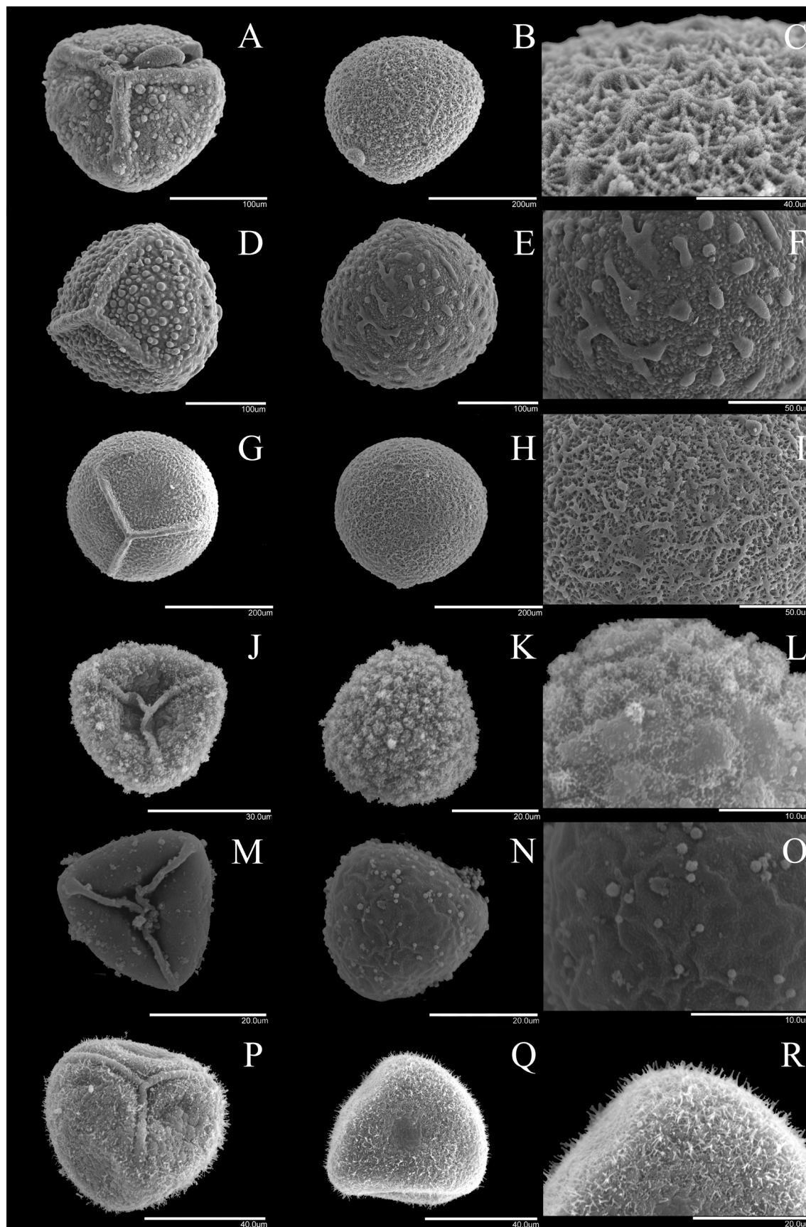
Fig. 2. Spore morphology of Selaginella kurzii (A–C – megaspores, J–L – microspores; F. G. Dickason 8164, LE); S. pseudorepanda (D–F – megaspores, M–O – microspores; S. Tagane et al. No. 304 (VNM00072393, paratype); S. repanda (G–I, P–R – megaspores, J–L – microspores; L. Averyanov et al. VH 1566 (LE); A, D, G, J, M, P – proximal face, B, E, H, K, N, Q – distal face, C, F, I, L, O, R – close-up of surface, distal face.
