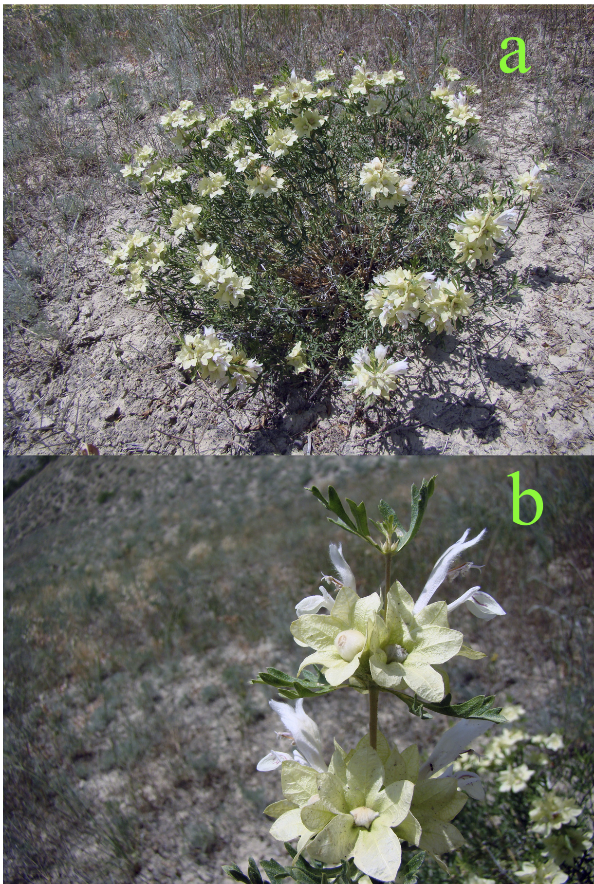
Fig. 1. Lagochilus ketmentubensis (plant in blossom from type location): a – general view; b – part of inflorescence.
